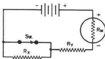
with Millimeter, Battery and Known Resistor
